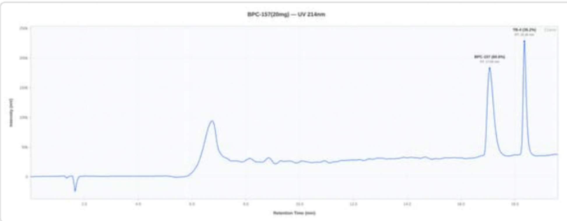
HPLC Chromatogram
