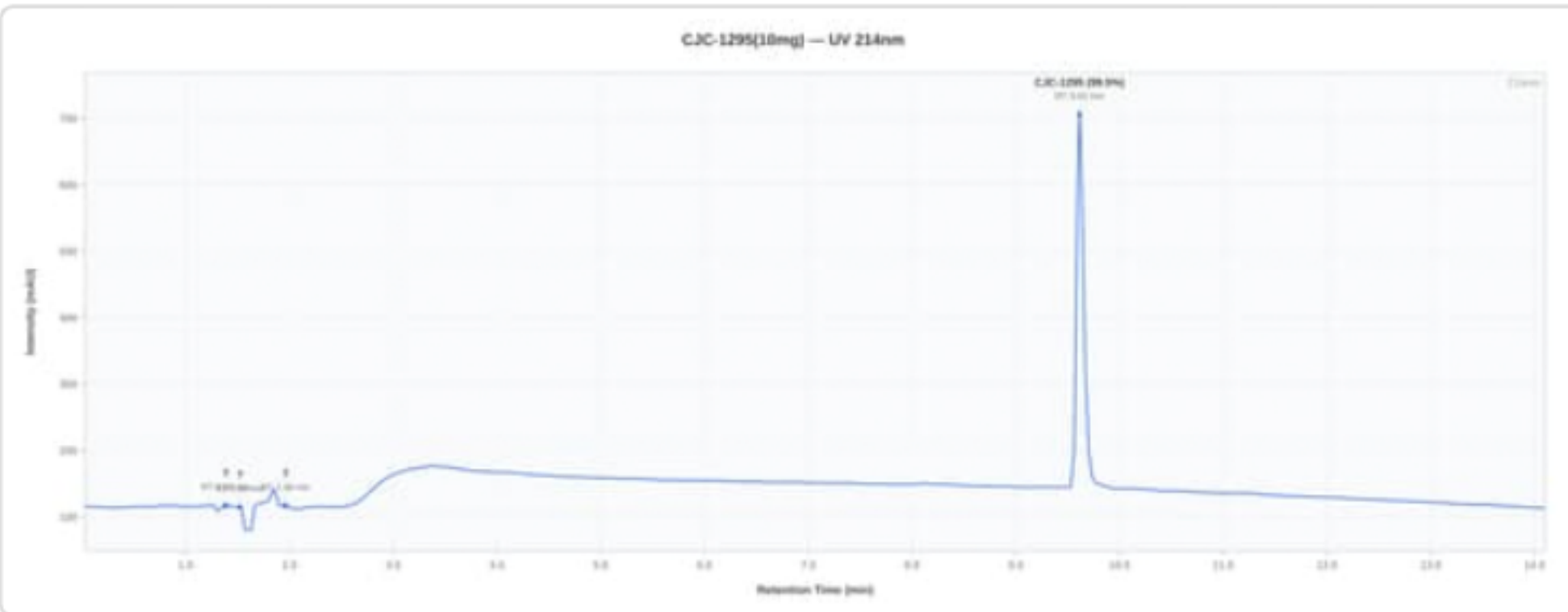
HPLC Chromatogram
