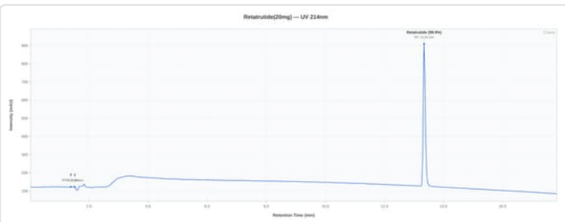
HPLC Chromatogram
