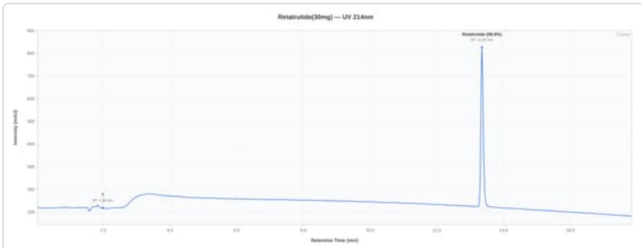
HPLC Chromatogram
