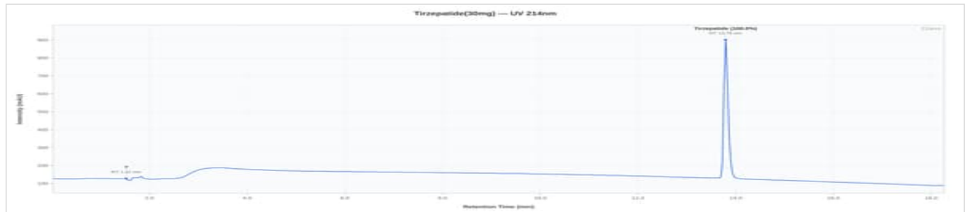
Tirzepatide 30mg - LOT-07062026TR30: UV Chromatogram
