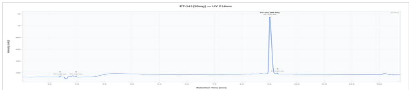
PT-141 10mg - 08242026-PT10: UV Chromatogram
