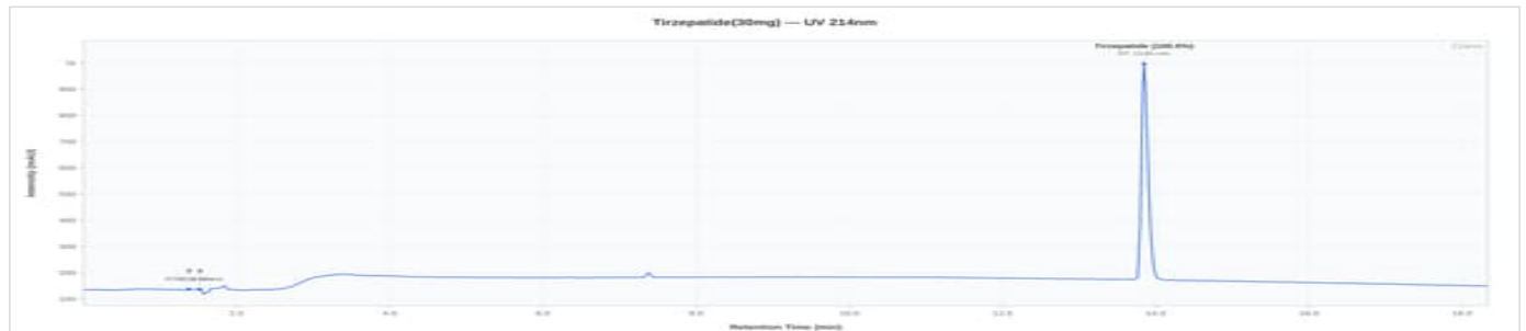
Tirzepatide 30mg - 08262026-TR30: UV Chromatogram
